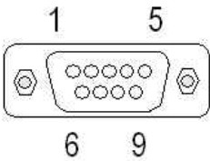
J9,J11: COM - 9-pin Dsub Connector
