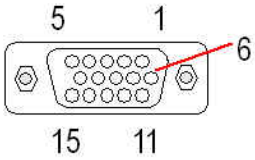
J15: VGA – 15-pin D-Sub Connector
